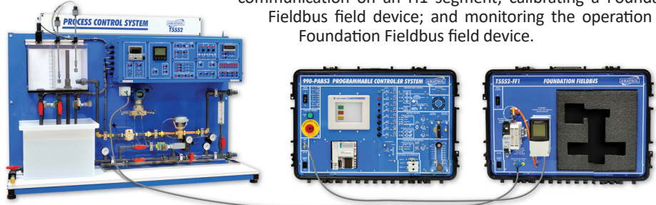
T5552-FF1 Foundation Fieldbus shown with T5552A and 990-PAB53
