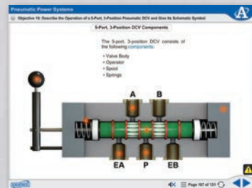
Pneumatic Power Systems
