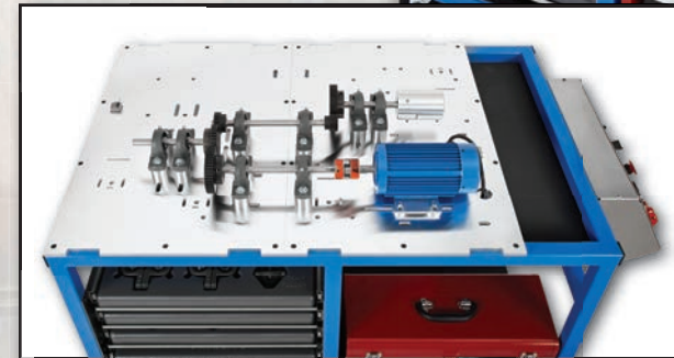
Mechanical Drives 1 Learning System (970-ME1)
